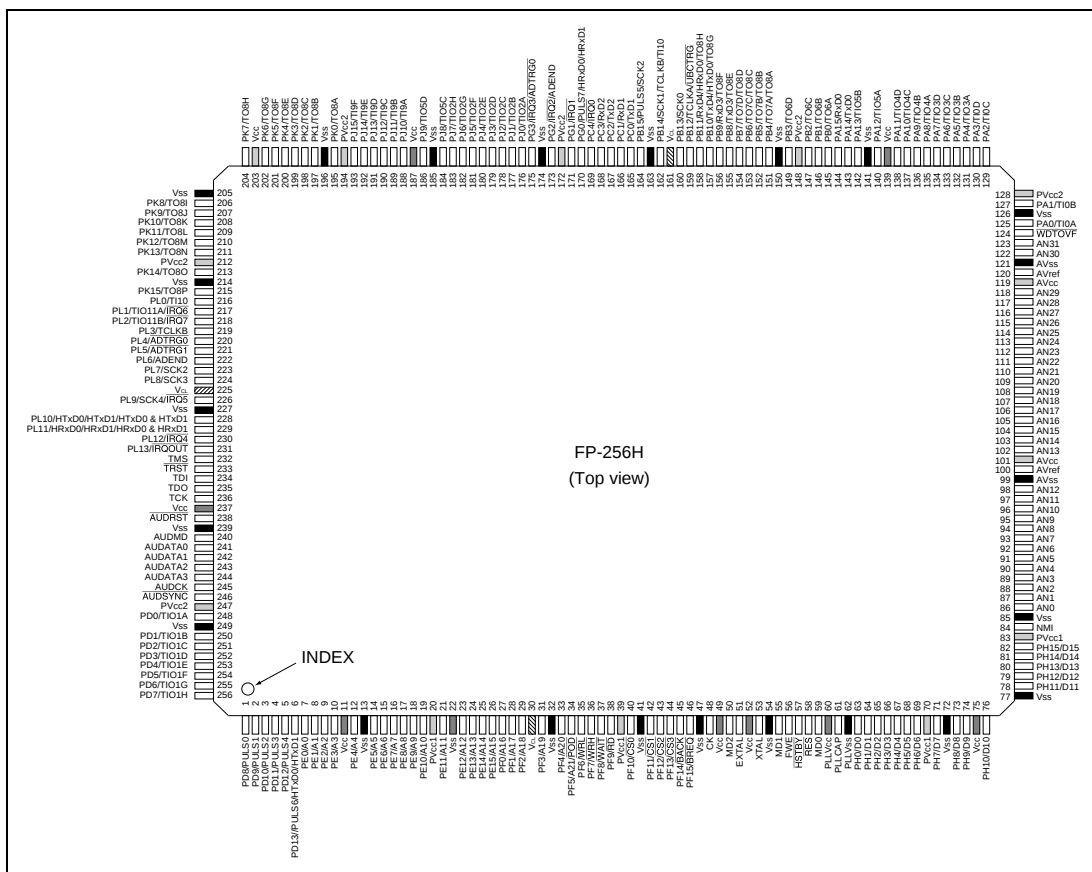
Figure 1.2 Pin Arrangement
