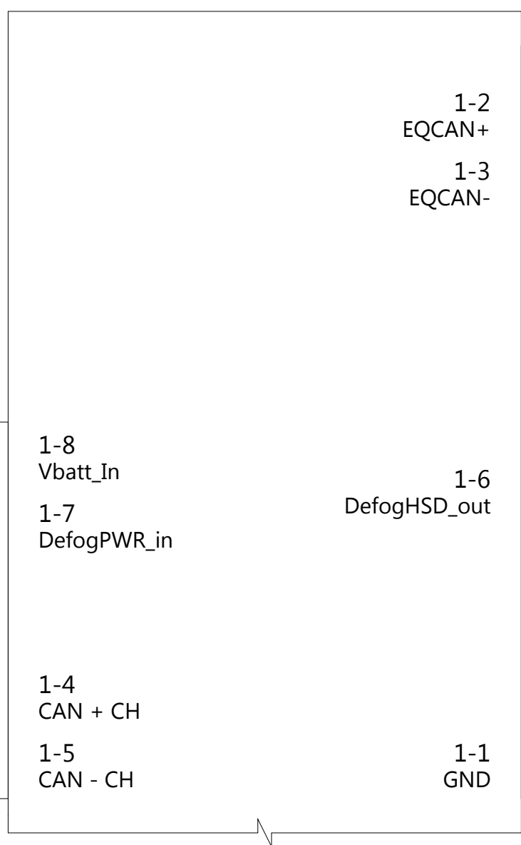
DA01 Forward Camera K X139
