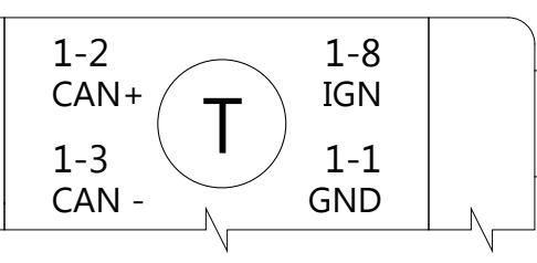
Radar Front L X138
