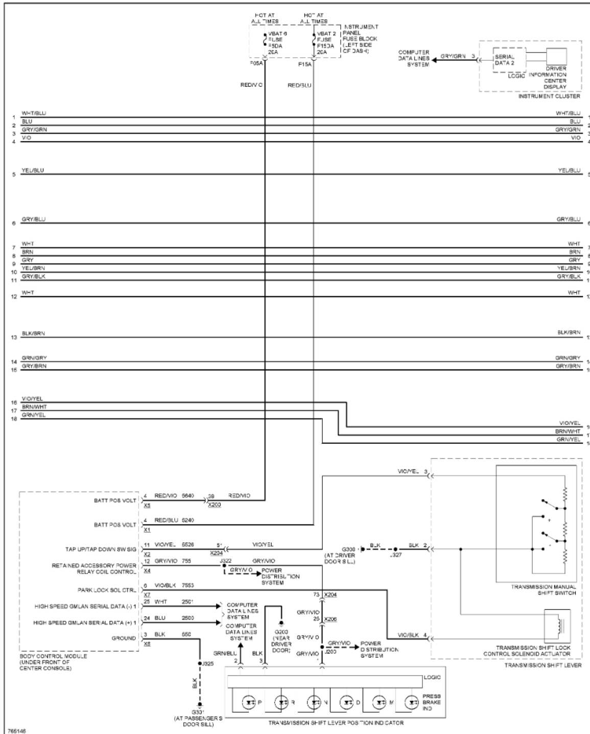
Fig. 136: A/T Circuit, 9 Speed (2 of 3)
