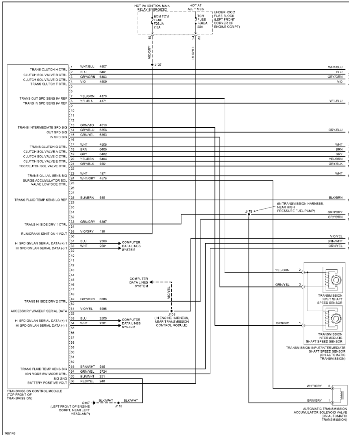
Fig. 135: A/T Circuit, 9 Speed (1 of 3)
