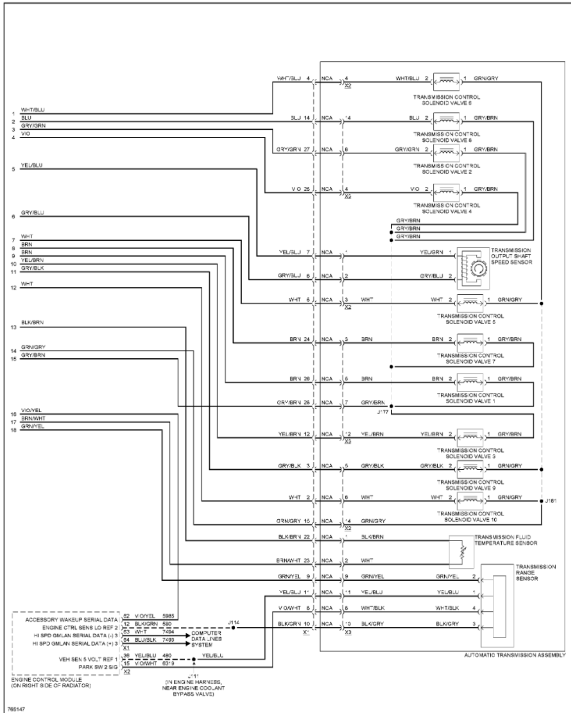
Fig. 137: A/T Circuit, 9 Speed (3 of 3)
